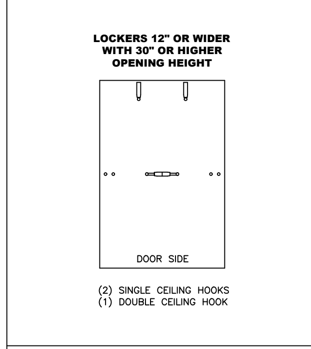
HOOK CONFIGURATION
