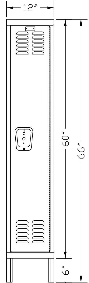
FRONT VIEW
