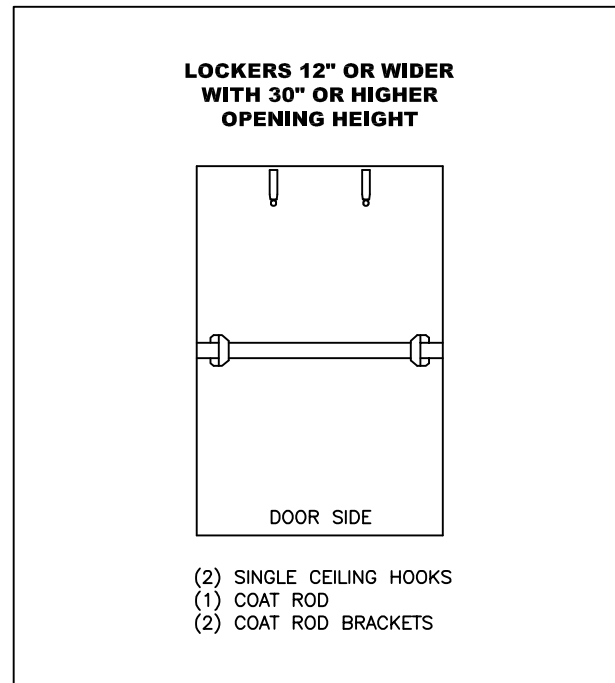
HOOK CONFIGURATION
