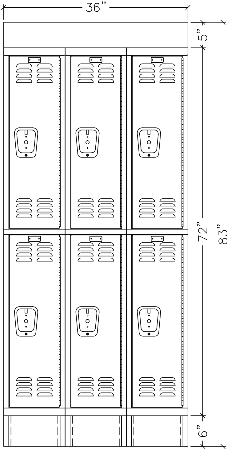
FRONT VIEW
