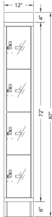
FRONT VIEW 1-WIDE
