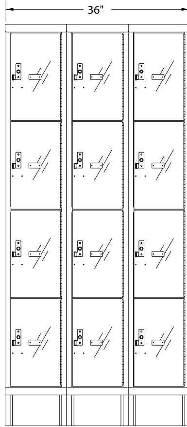
FRONT VIEW 3-WIDE
