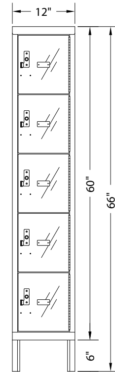
FRONT VIEW
