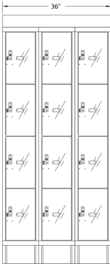
FRONT VIEW 3-WIDE
