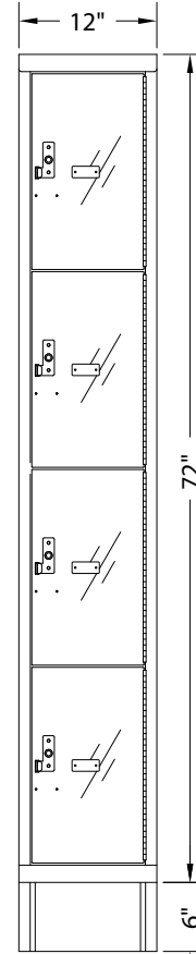
FRONT VIEW 1-WIDE
