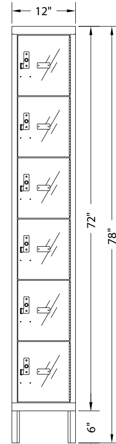
FRONT VIEW
