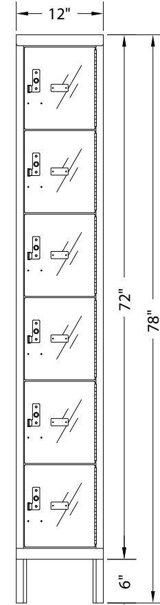
FRONT VIEW
